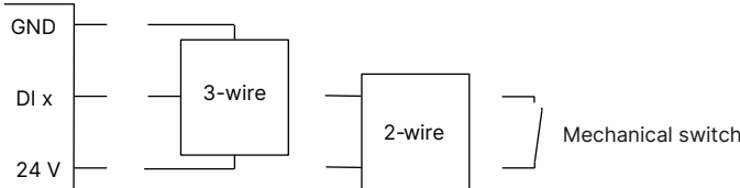
Circuit diagram:
