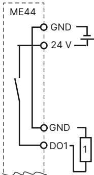
Circuit diagram:
